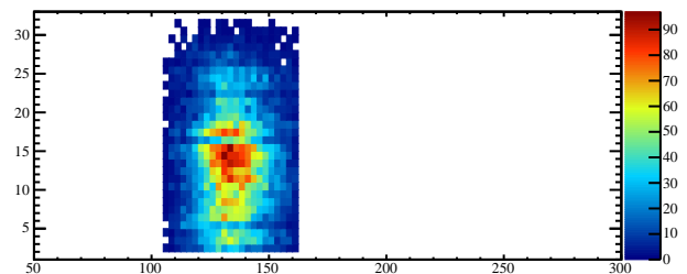
Mass vs x-2
