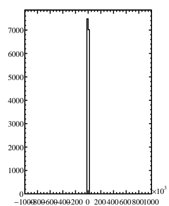
fMassBiasHist
