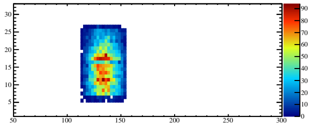
Mass vs x-27
