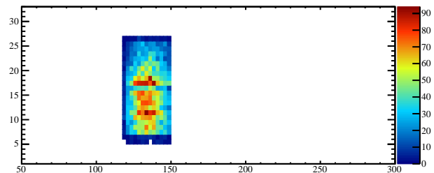
Mass vs x-39
