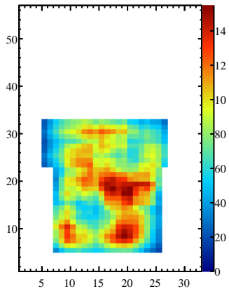
Bigalcal Event Energy
