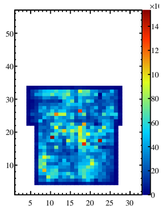
Bigalcal P10 Event Clusters
