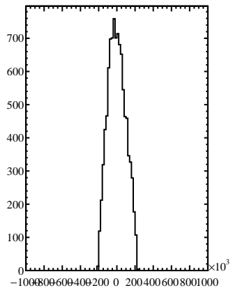
fMassBiasHist
