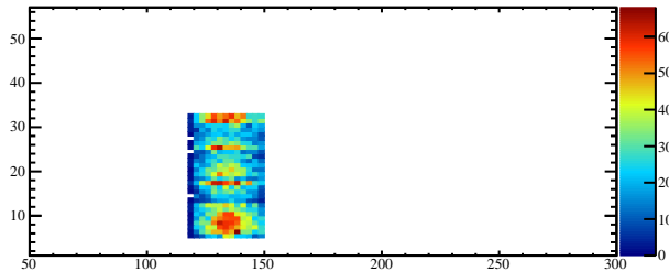
YvsMass-13
