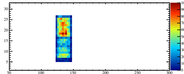
Mass vs x-19
