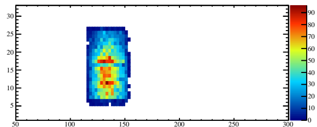
Mass vs x-9
