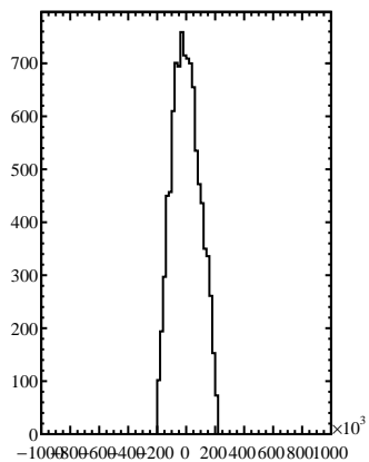
fMassBiasHist
