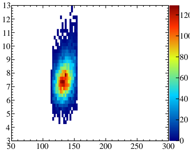
AnglesvsMass-14
