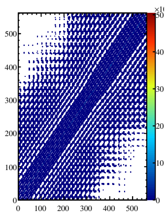
C matrix
