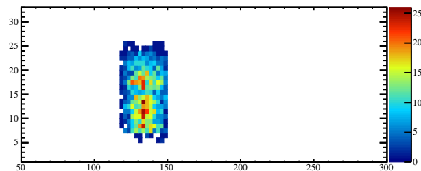
Mass vs x-13
