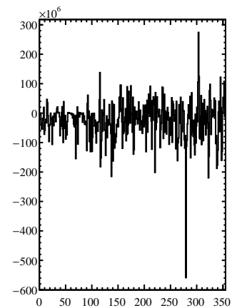
D Vector
