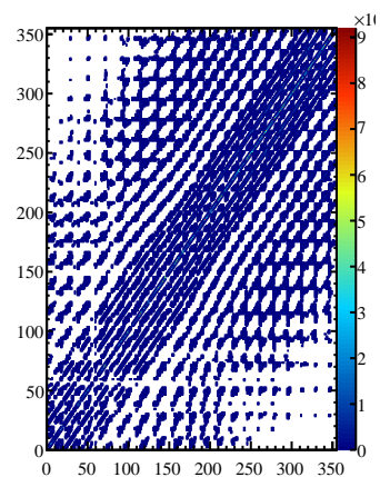
C matrix
