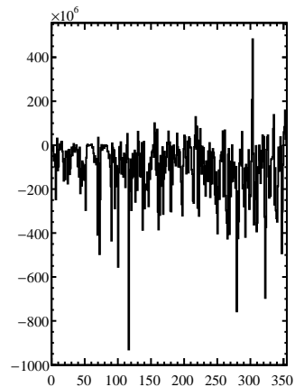
D Vector
