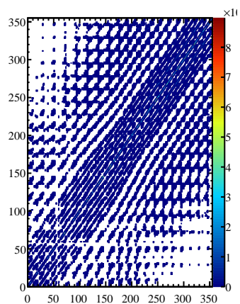
C matrix
