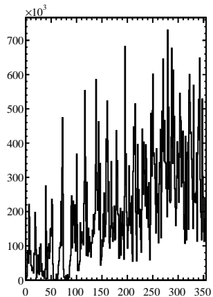
L Vector
