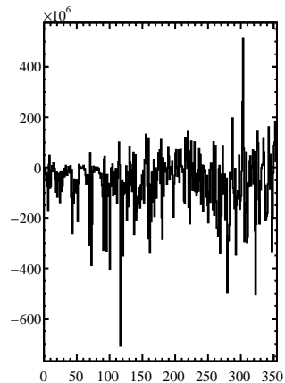
D Vector
