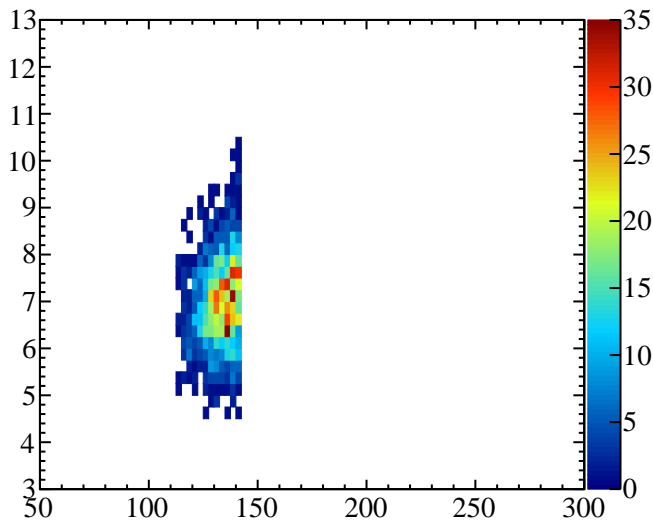
AnglevsMass-9
