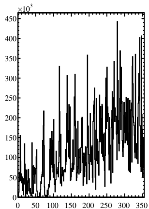
L Vector
