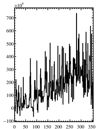
D Vector
