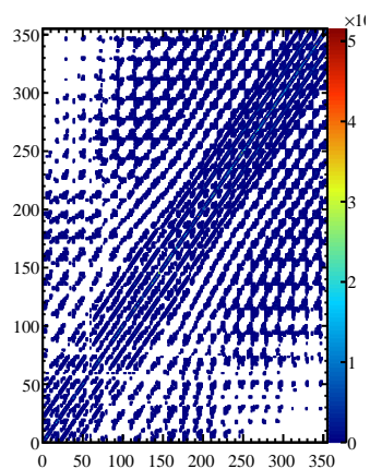
C matrix
