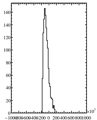
fMassBiasHist
