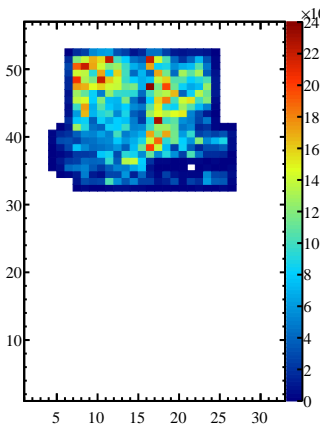
Bigal P0 Event Clusters
