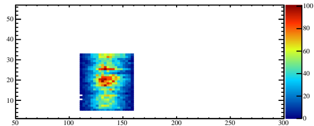
YvsMass-6
