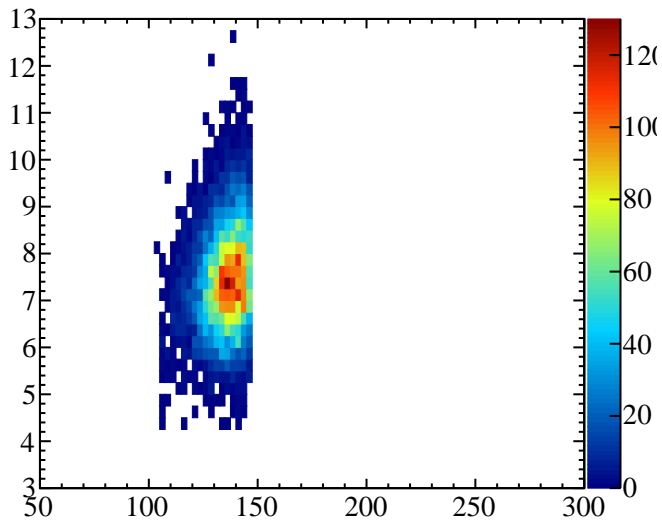
AnglevsMass-8
