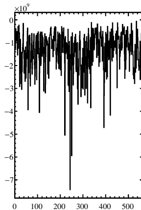
D Vector
