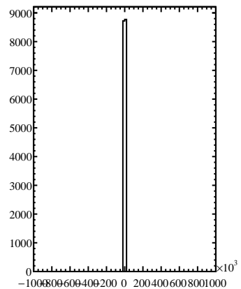
fMassBiasHist
