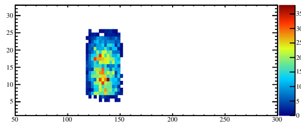
Mass vs x-13
