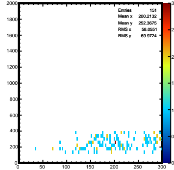
nu vs \pi mass
