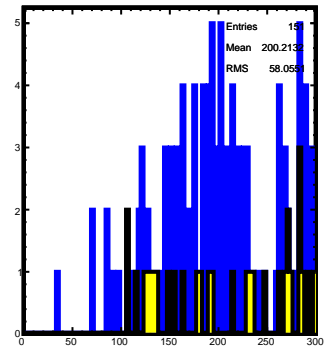
Mass (good GammaStar)
