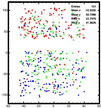
Positron position
