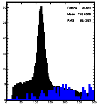
\pi^0 Mass
