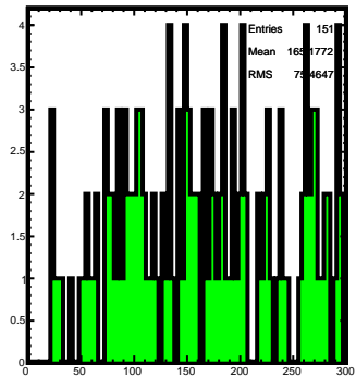
Gamma mass
