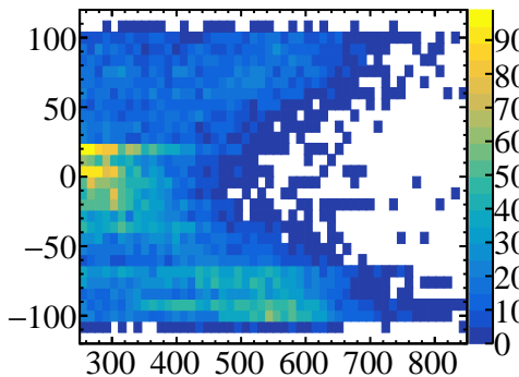
massVSy1
