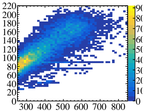
massVSD
