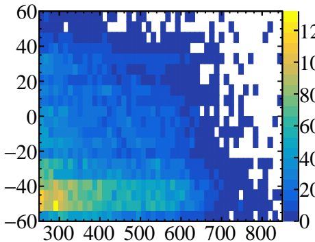
massVSx1
