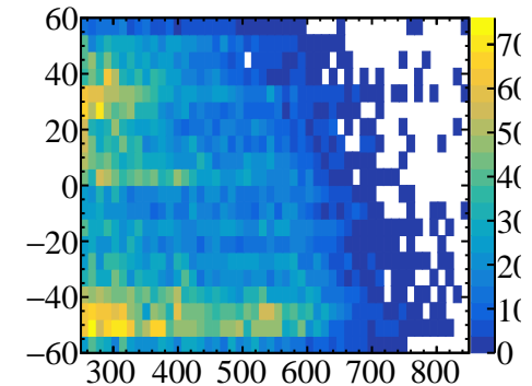
massVSx2
