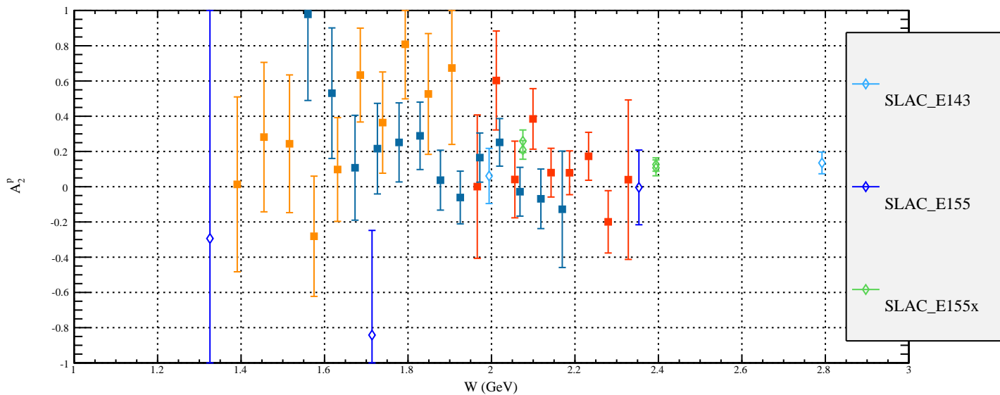
Preliminary A_2^P , E=4.7 GeV
