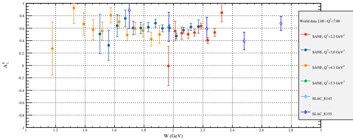
Preliminary A_1^P , E=4.7 GeV
