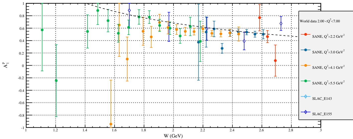
Preliminary A_1^P , E=5.9 GeV
