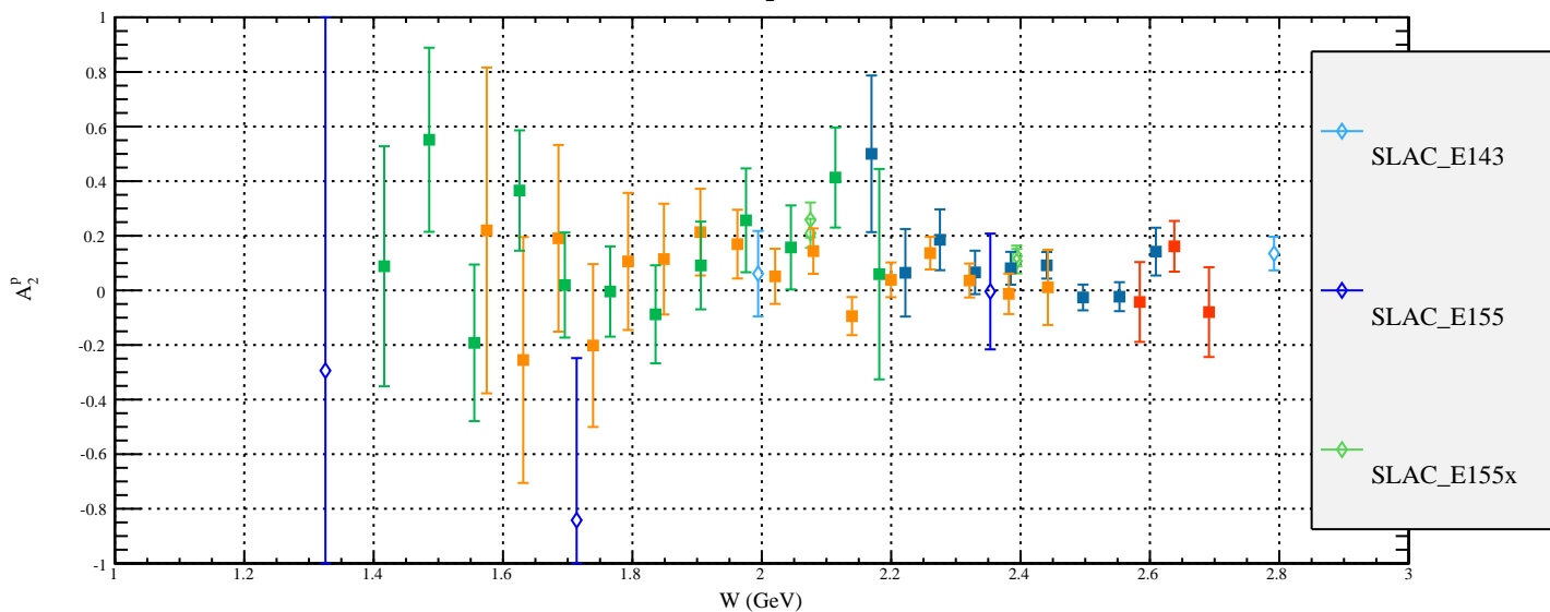
Preliminary A_2^P , E=5.9 GeV
