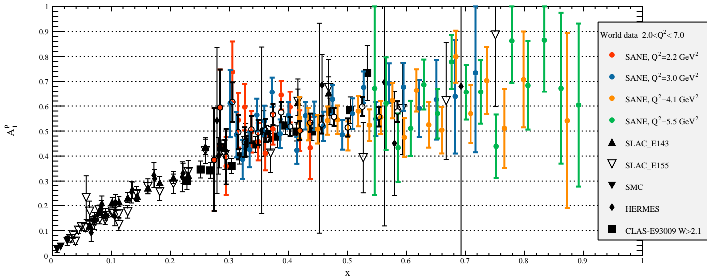
Preliminary A_1^P , Combined Beam Energies
