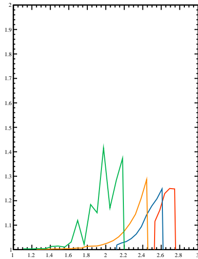
C_{bg}
