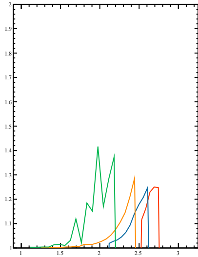
1/f_{bg}
