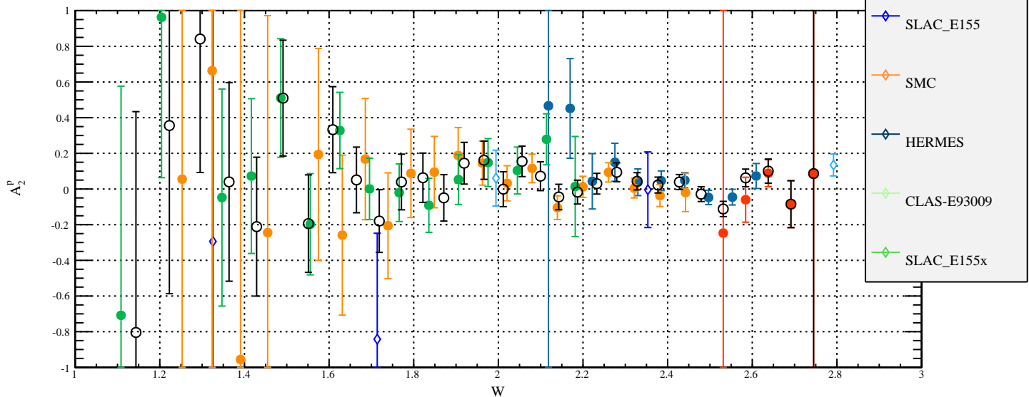
Preliminary A_2^p , E=5.9 GeV
