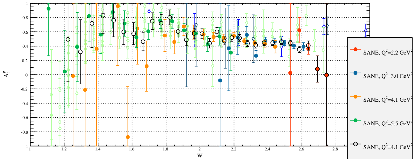
Preliminary A_1^p , E=5.9 GeV
