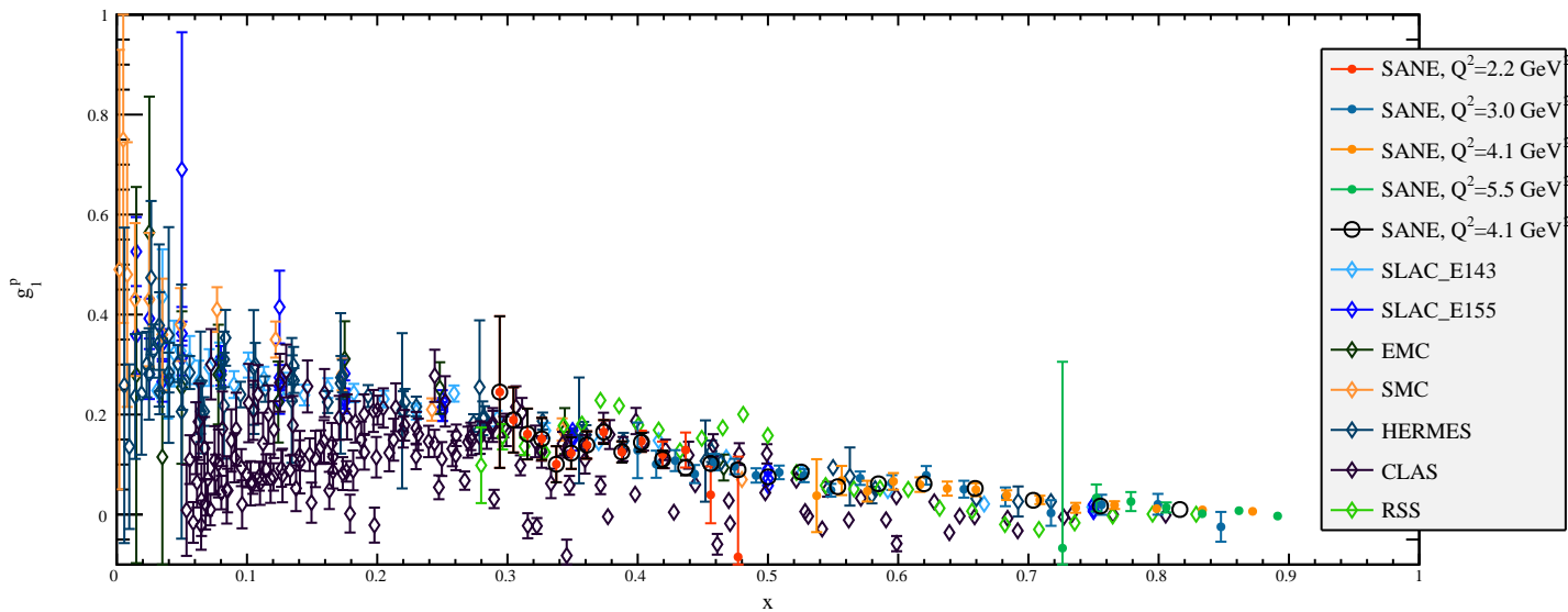
Preliminary g_1^p , E=4.7 GeV
