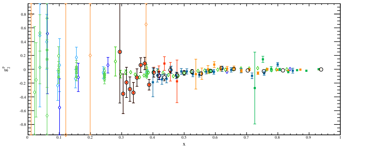
Preliminary g_2^p , E=4.7 GeV
