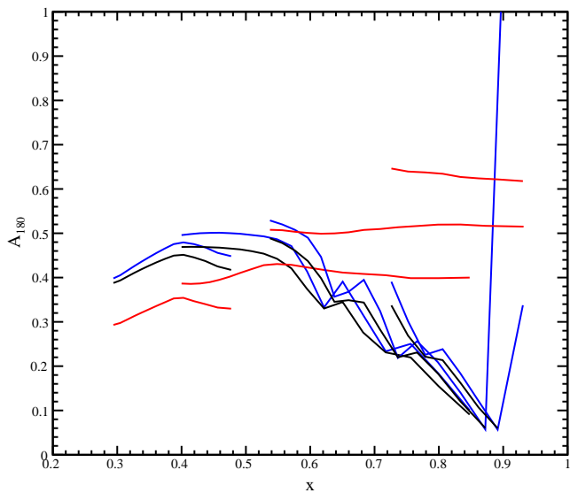
A_{180}, E=4.7 \text{ GeV}
