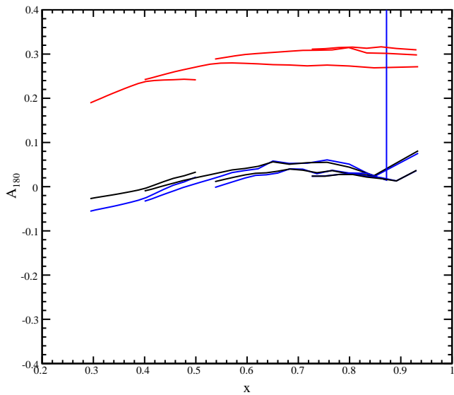
A_{80}, E=4.7 \text{ GeV}
