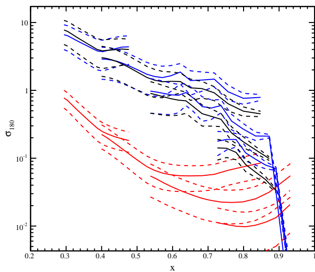
\sigma_{180}, E=4.7 \text{ GeV}
