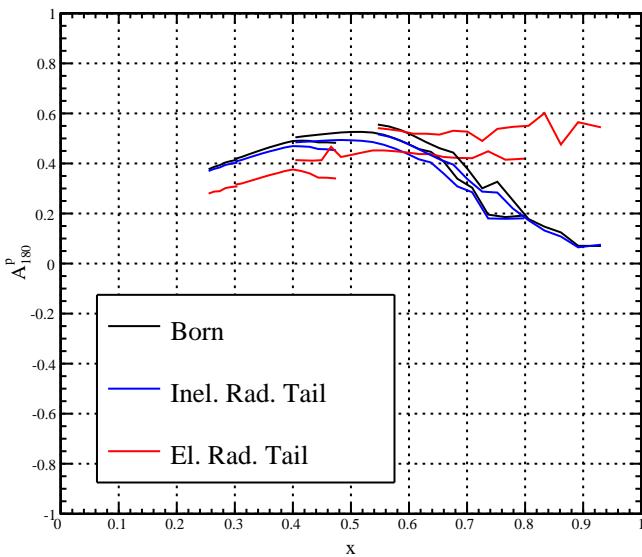
A_{180}^P, E=5.9 \text{ GeV}
