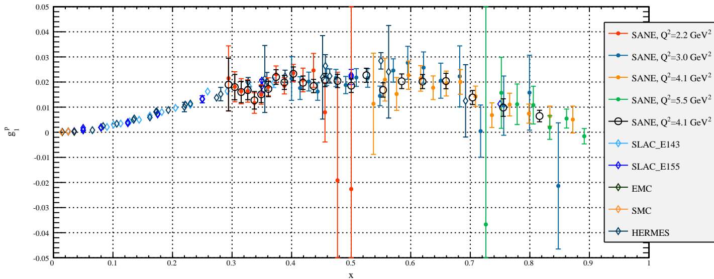
Preliminary g_1^p , E=4.7 GeV
