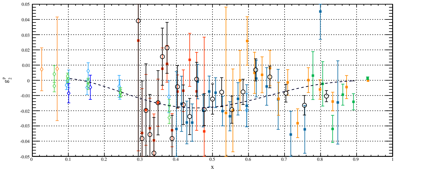
Preliminary g_2^p , E=4.7 GeV
