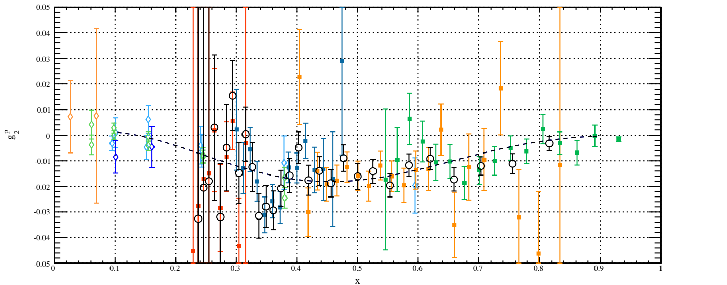
Preliminary g_2^p , E=5.9 GeV
