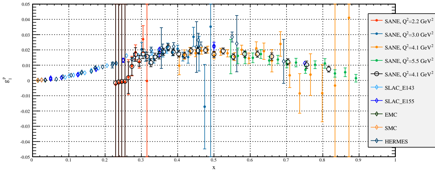
Preliminary g_1^p , E=5.9 GeV
