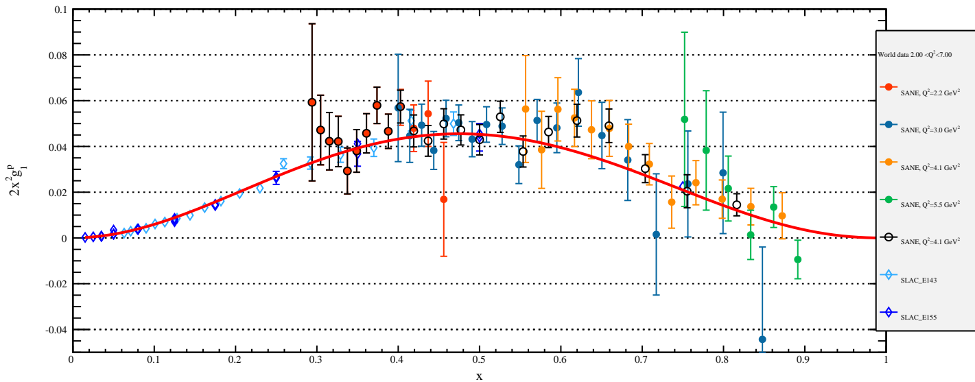
Preliminary 2x^2g_1^p , E=4.7 GeV
