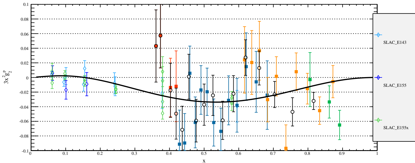
Preliminary 3x^2g_2^p , E=4.7 GeV
