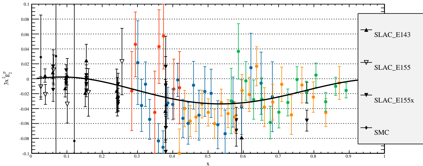
Preliminary 3x^2g_2^p , Combined Beam Energies
