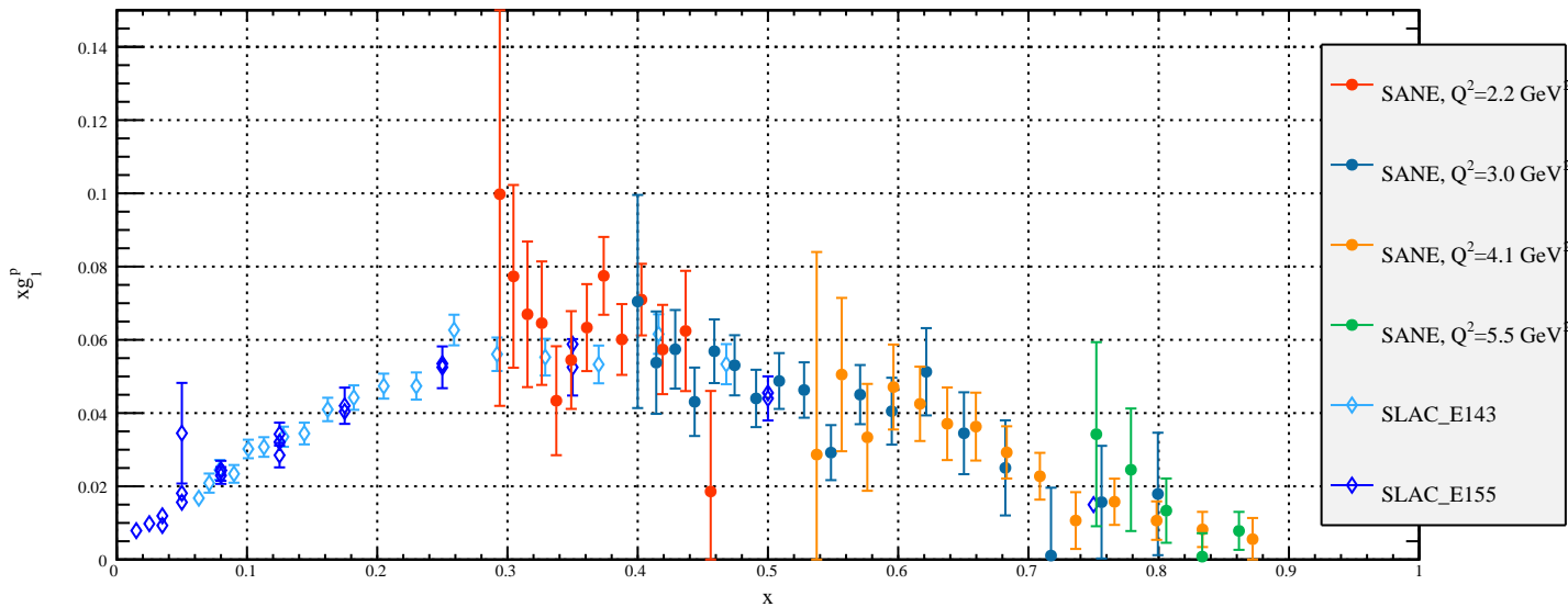
Preliminary xg_1^p , E=4.7 GeV
