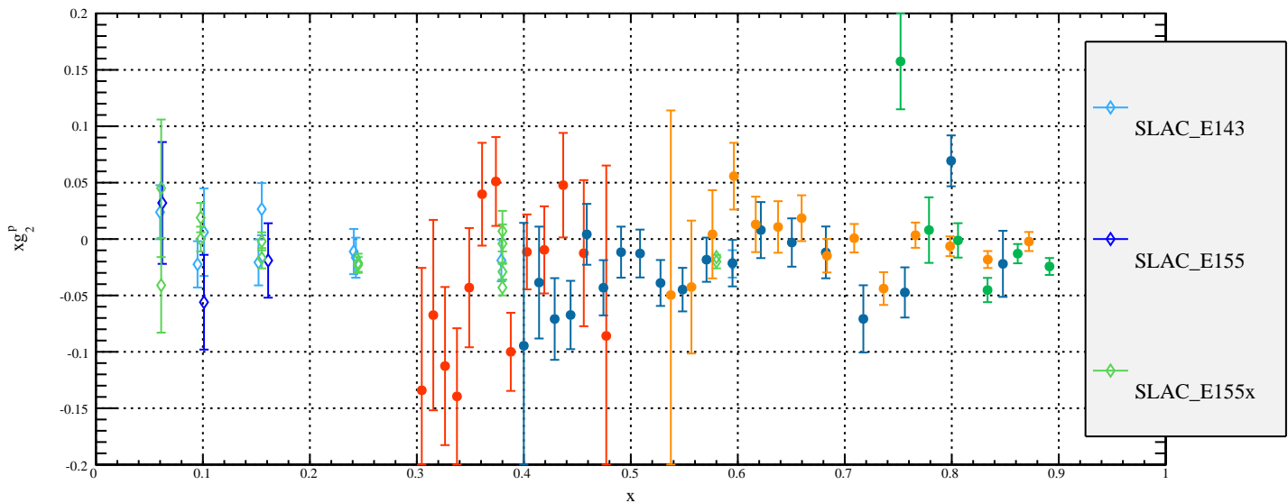
Preliminary xg_2^p , E=4.7 GeV
