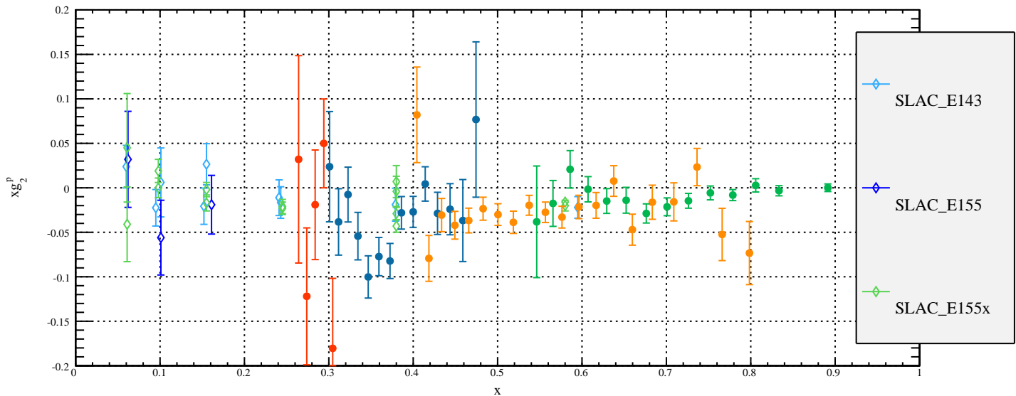
Preliminary xg_2^p , E=5.9 GeV
