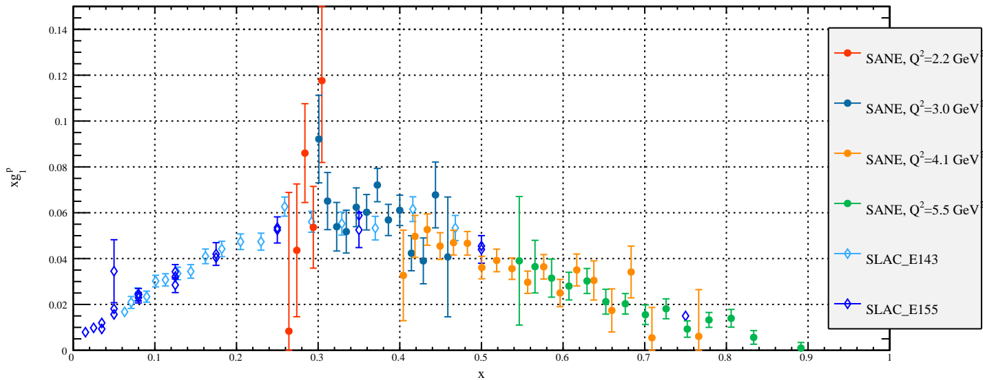
Preliminary xg_1^p , E=5.9 GeV
