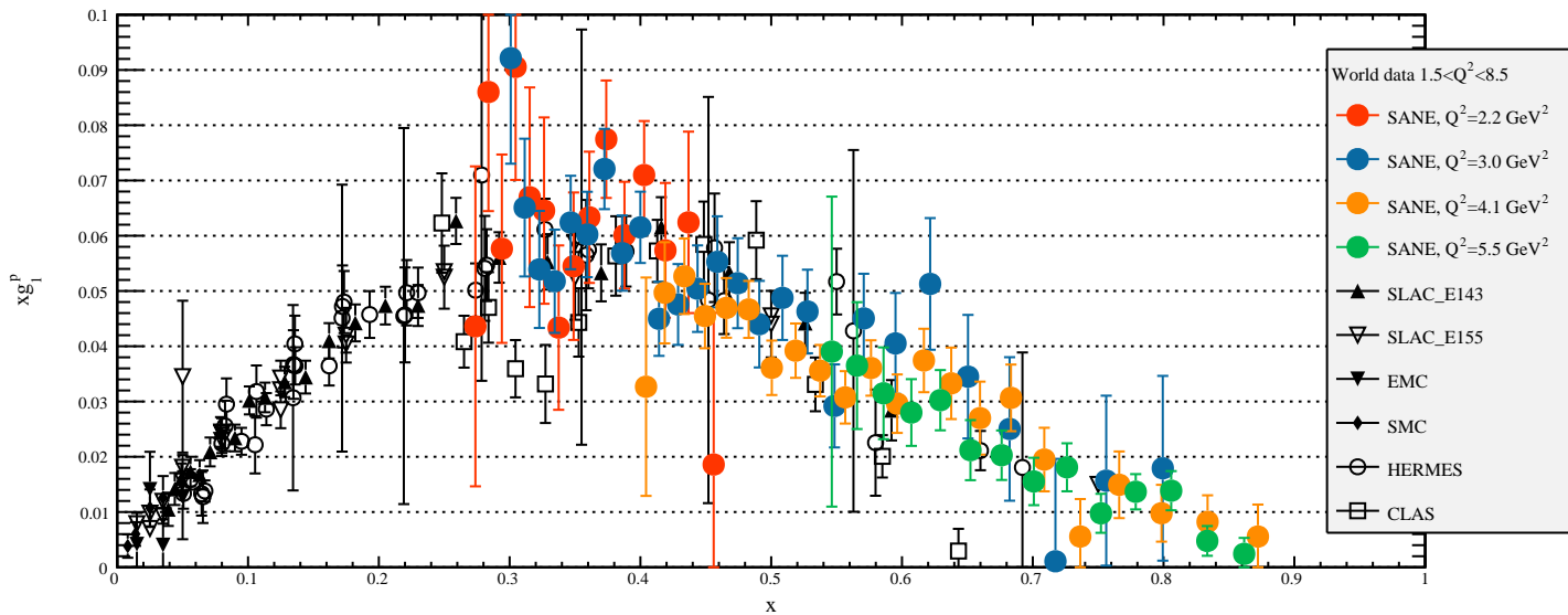
Preliminary xg_1^p , Combined Beam Energies
