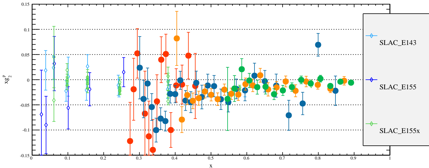
Preliminary xg_2^p , Combined Beam Energies
