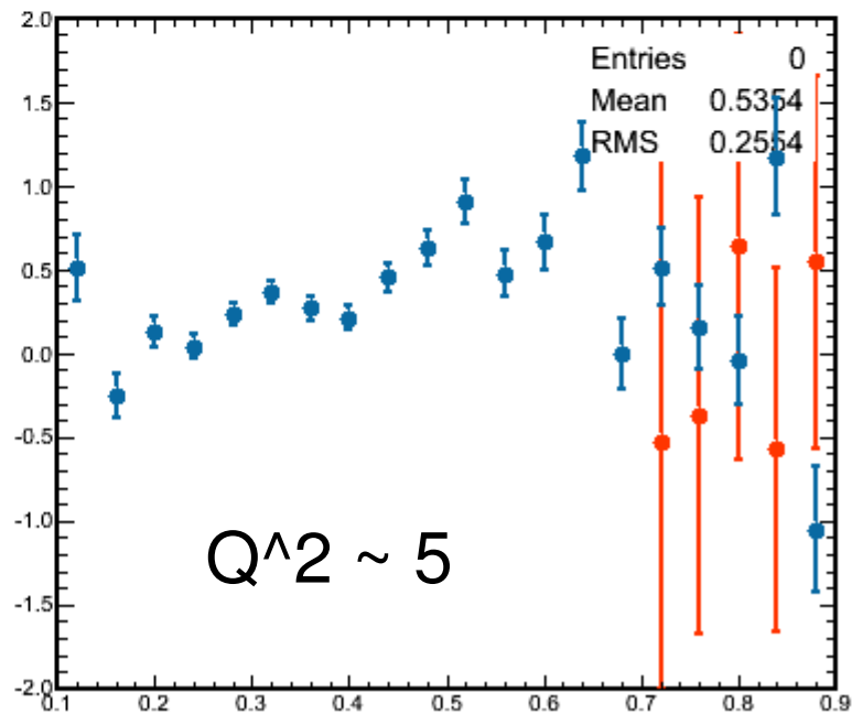
Physics Asymmetry
