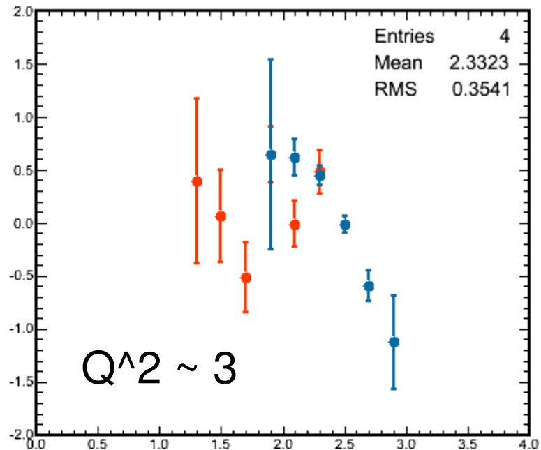
Physics Asymmetry
