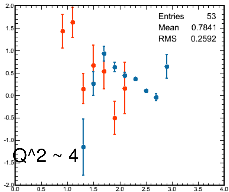
Physics Asymmetry
