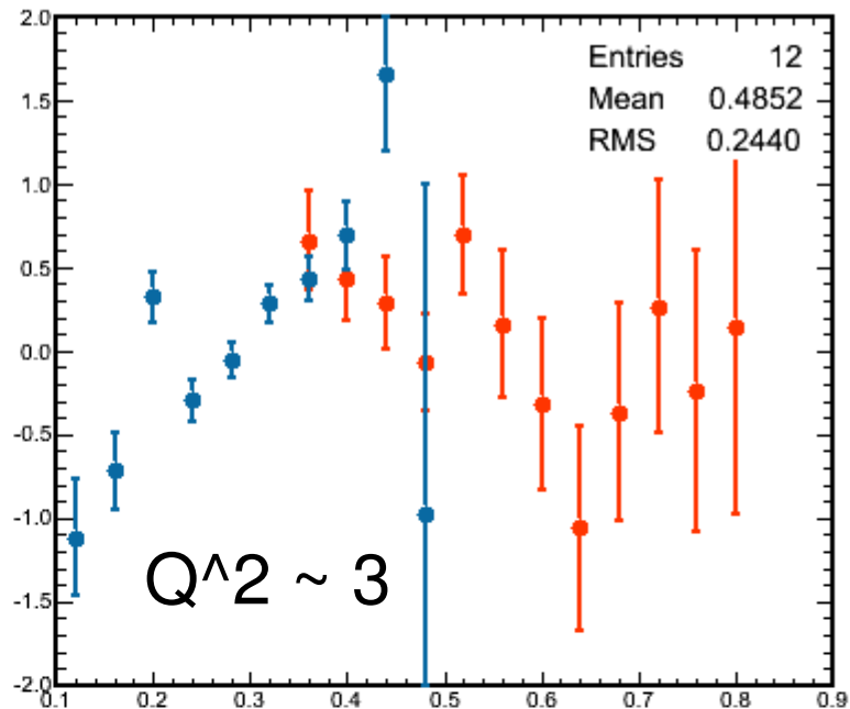
Physics Asymmetry
