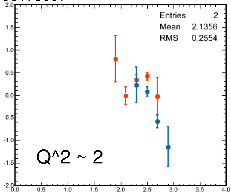
72999+73001 Physics Asymmetry
