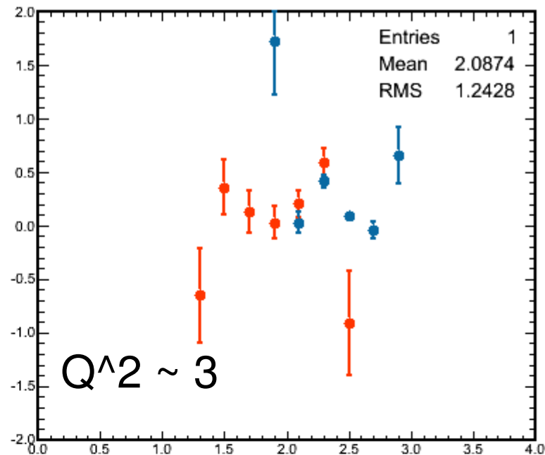
Physics Asymmetry
