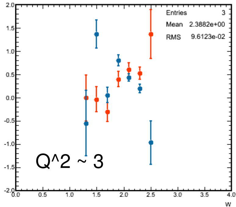
Physics Asymmetry
