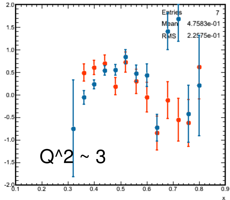
Physics Asymmetry
