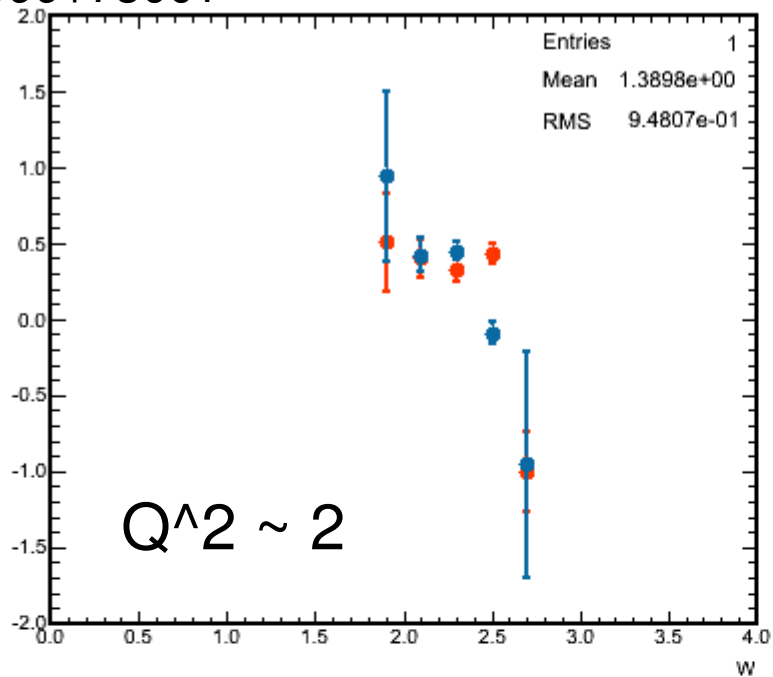
72999+73001 Physics Asymmetry
