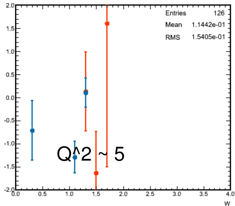
Physics Asymmetry
