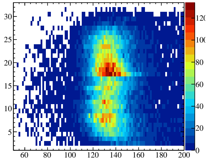
Mass vs x-0
