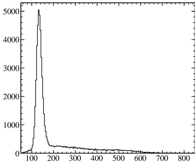
\eta mass
