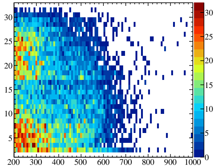
\eta Mass vs x-0
