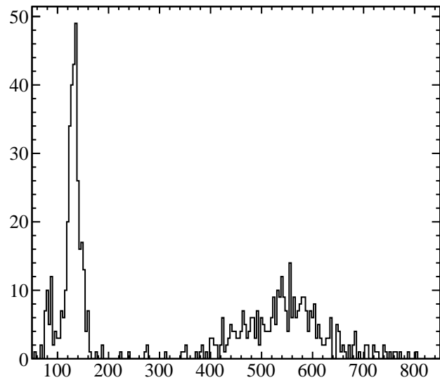
\eta mass
