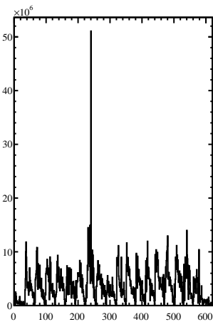
L Vector
