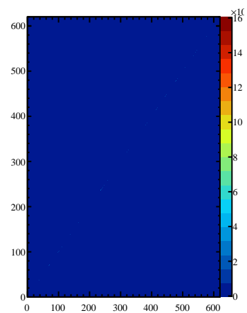
C matrix
