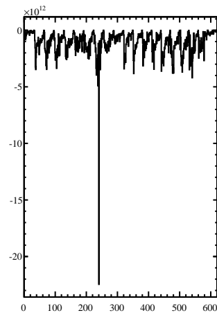
D Vector
