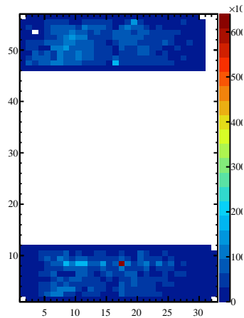
Bigcal Pi0 Event Clusters
