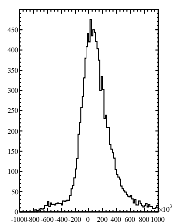
fMassBiasHist
