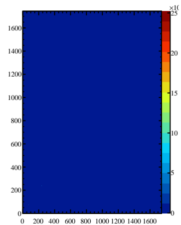
C matrix
