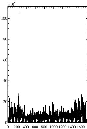
L Vector
