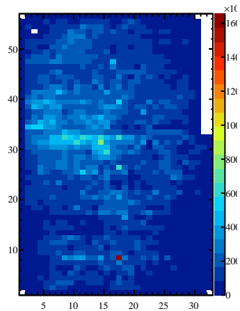
Bigcal Pi0 Event Clusters
