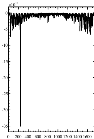
D Vector
