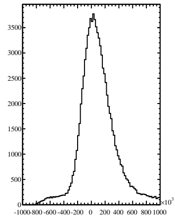
fMassBiasHist
