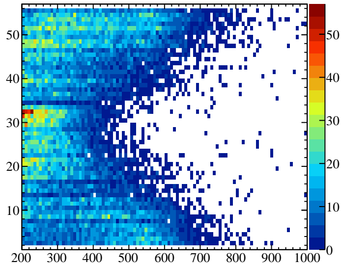
\eta YvsMass-0
