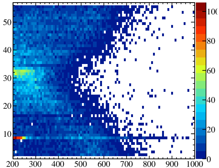
\eta YvsMass-0
