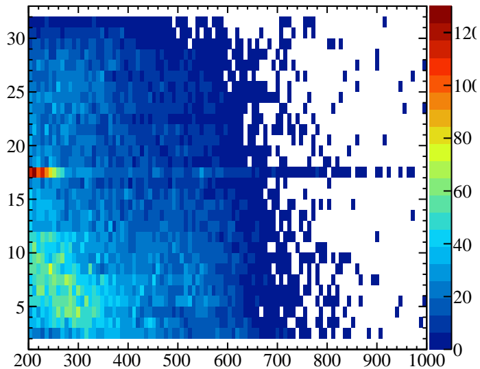
\eta Mass vs x-0
